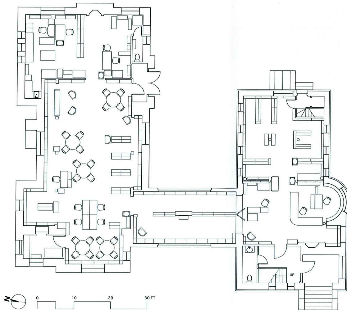
HOPKINTON PUBLIC LIBRARY FIRST FLOOR
